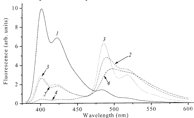
Figure 6. Fluorescence spectra of a mixture of non-complementary modified oligonucleotides 23 and 29 (1), and duplexes 23 · 33 (2), 26 · 33 (3), and 24 · 34 (4); \lambda_{\text{ex}} = 370 nm
