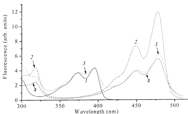
Figure 7. Excitation spectra of modified oligonucleotides 23 (1), 29 (2), and duplexes 23 · 33 (3), 29 · 33 (4), \lambda_{\text{em}} = 520 nm
