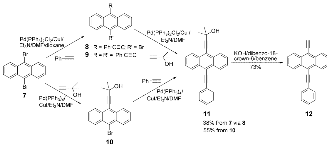
Scheme 2. Preparation of alkyne derivative 12
