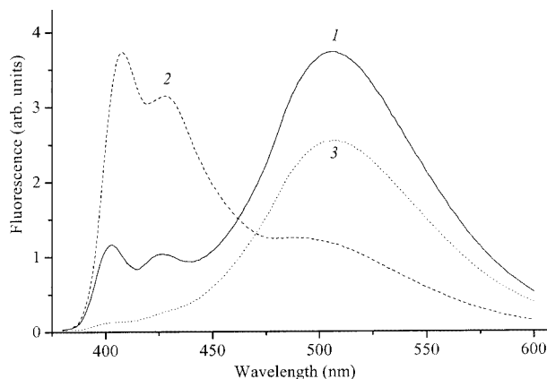
Figure 4. Fluorescence spectra of modified oligonucleotide 24 (1) and duplexes 22 · 24 (2) and 22 · 25 (3); \lambda_{\text{ex}} = 370 nm
