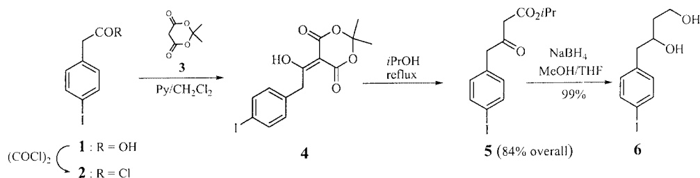
Scheme 1. Preparation of (iodophenyl)-diol 6
