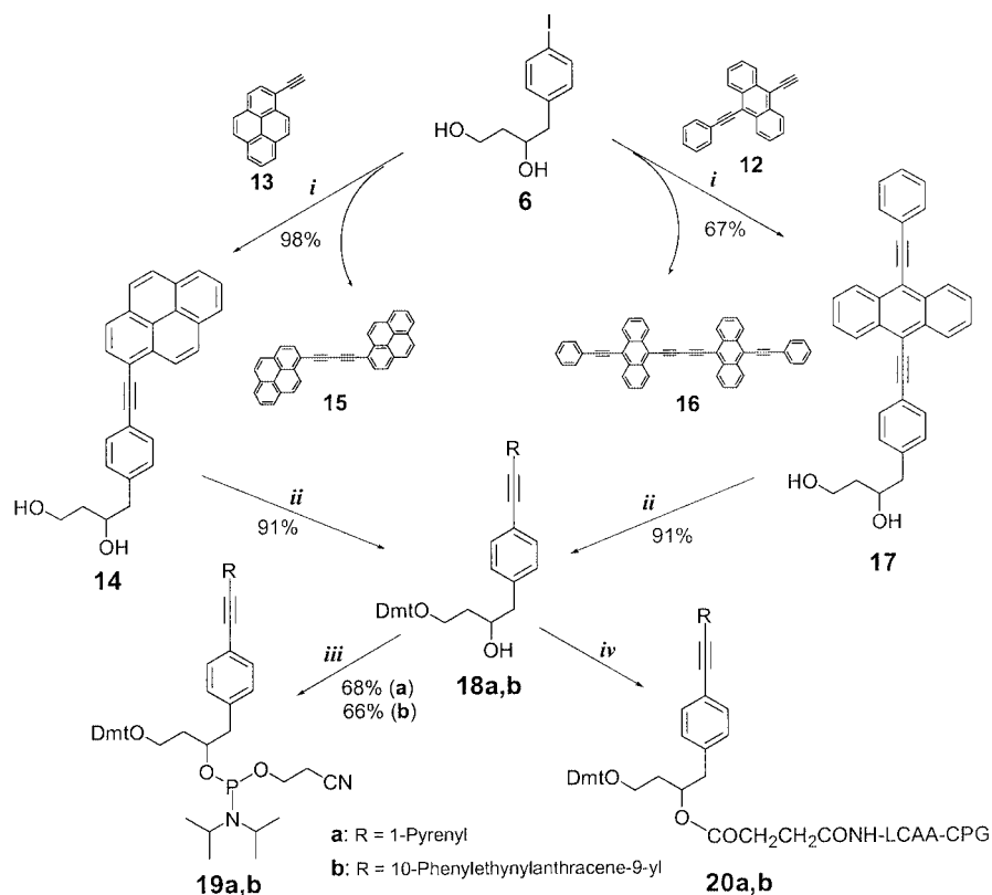
Scheme 3. Preparation of PEPy and BPEA phosphoramidites and solid supports; reagents: i: [\text{Pd}(\text{PPh}_3)_4]/\text{CuI}/\text{Et}_3\text{N}/\text{DMF} ; ii: \text{DmtCl}/\text{Py} ; iii: (i\text{Pr}_2\text{N})_2\text{POCH}_2\text{CH}_2\text{CN}/\text{diisopropylammonium tetrazolide}/\text{MeCN} ; iv: \text{LCAA-CPG-NHCOCH}_2\text{CH}_2\text{CO}_2\text{H}/N,N' -diisopropylcarbodiimide/ \text{DMAP}/\text{DMF}
