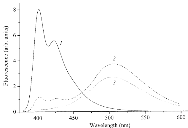
Figure 2. Fluorescence spectra of modified oligonucleotides 23 (1), 24 (2), and 25 (3); \lambda_{\text{ex}} = 370 nm
