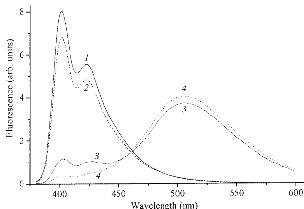
Figure 3. Fluorescence spectra of modified oligonucleotides 23 (1) and 24 (3), and duplexes 23 · 27 (2) and 24 · 28 (4); \lambda_{\text{ex}} = 370 nm
