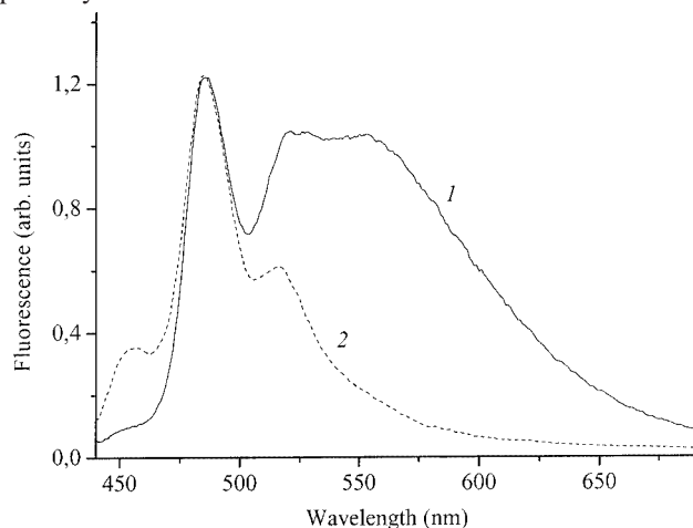
Figure 5. Fluorescence spectra of modified duplexes 29 · 33 (1) and 30 · 34 (2); \lambda_{\text{ex}} = 430 nm
