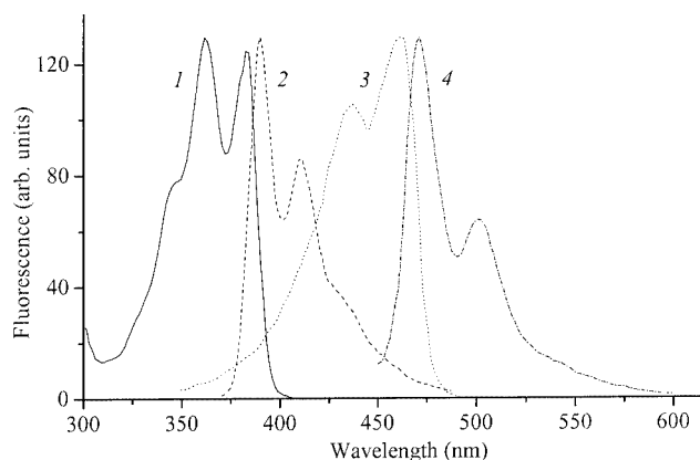
Figure 1. Normalized excitation spectra of diols 14 (1, \lambda_{\text{em}} = 440 nm) and 17 (3, \lambda_{\text{em}} = 520 nm), and fluorescence spectra of 14 (2, \lambda_{\text{ex}} = 320 nm) and 17 (4, \lambda_{\text{ex}} = 400 nm) in MeOH ( 10^{-6} M)
